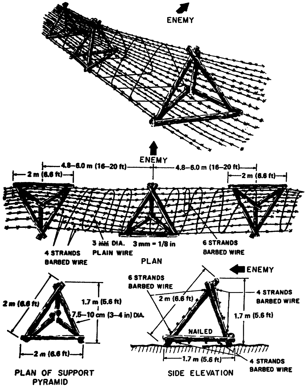
Figure 4-32. Lapland fence.
